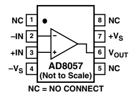
R-8 (SOIC)
